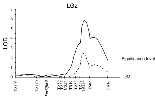
Fig. 2 QTL for ascochyta blight resistance obtained in the chickpea RIL population ILC3279 × WR315 evaluated in 2002 (—) and 2003 (---). Fusarium wilt race 5 resistant gene is in bold , the SCAR marker is underlined and the remainder of the markers are STMS
